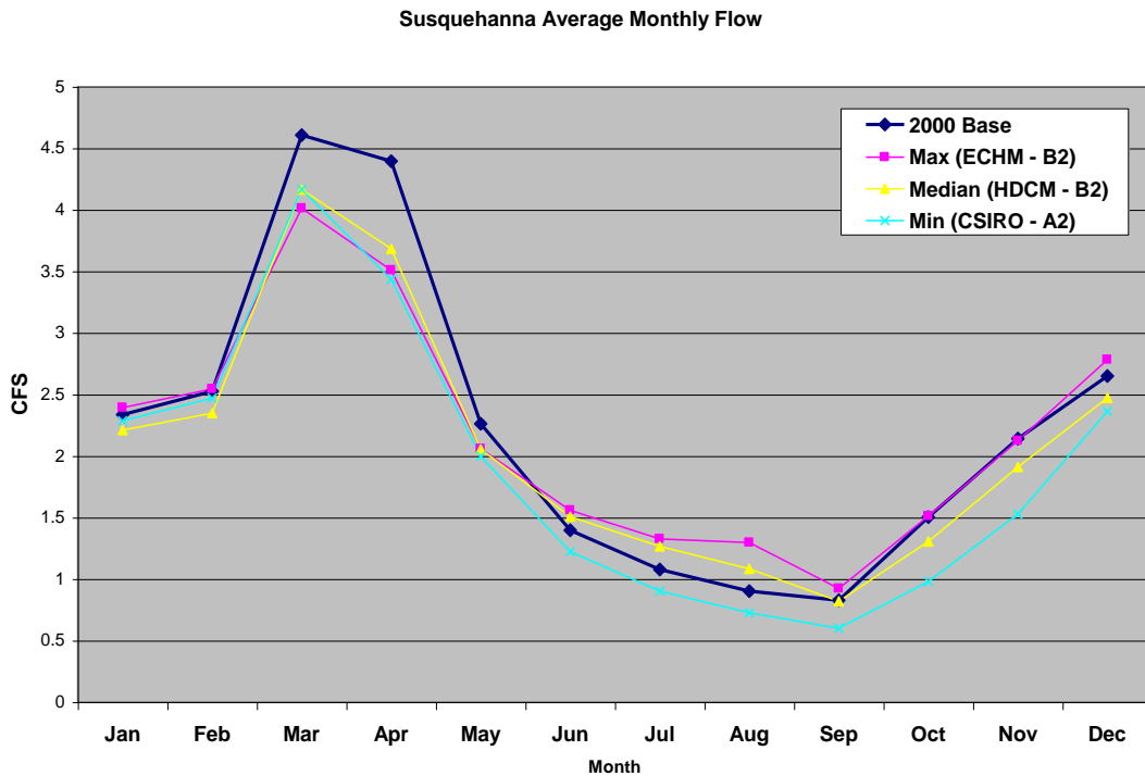
Figure E-1. Average annual time series of flow (cubic feet per second) for the 2000 Base Scenario and the maximum, median, and minimum climate change scenarios.
